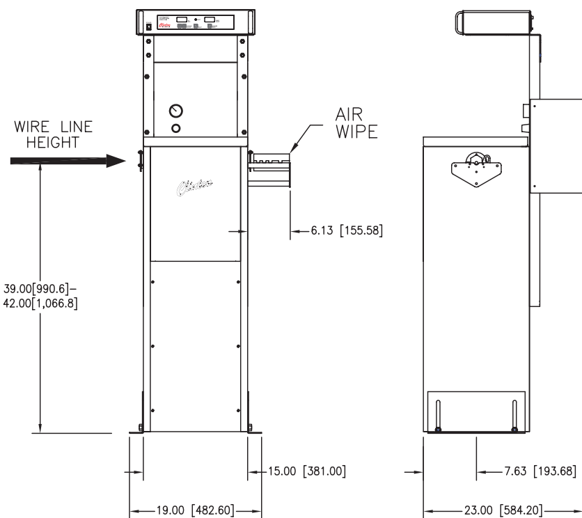
CONTROL UNIT
